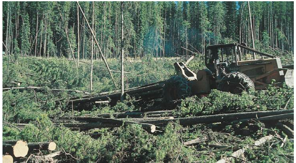
Skidders or dozers drag logs from the forest to the log landing. To reduce soil disturbance, rubber-tired skidders or crawler tractors should be kept on skid trails. Winch line and chokers pull logs to the machine.
