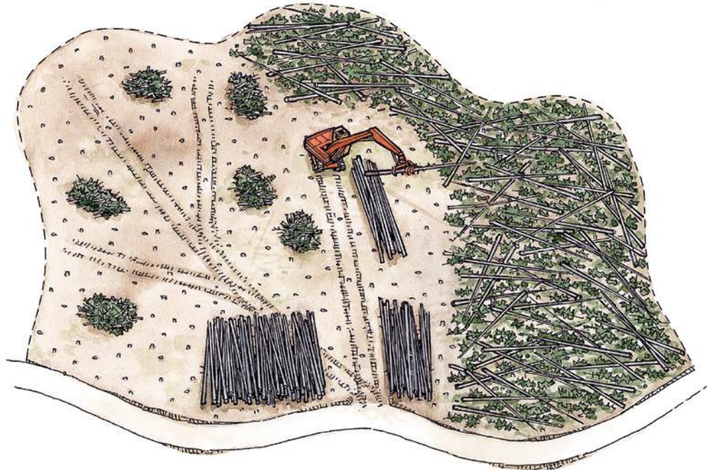
Shovel logging starts at the nearest access point and moves logs until they are within reach of the road. From there, they can be loaded onto trucks.
